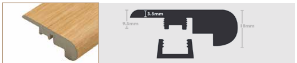
Stair Nosing
