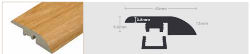
Ramp Profile
