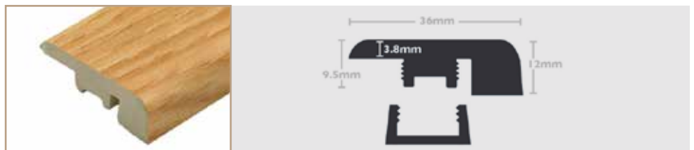
End Profile
